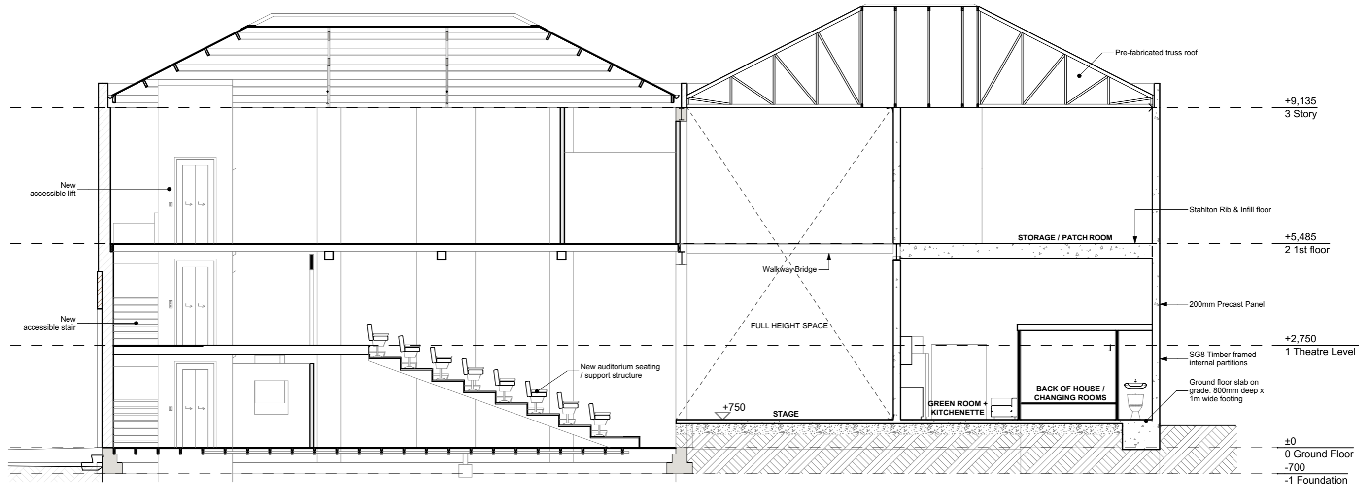
a-a Section Proposed 1:100
